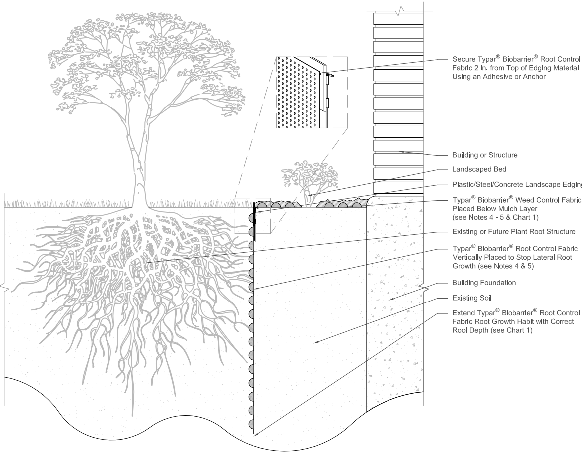
1 Biobarrier® : Foundation Protection Application Scale : N.T.S.
